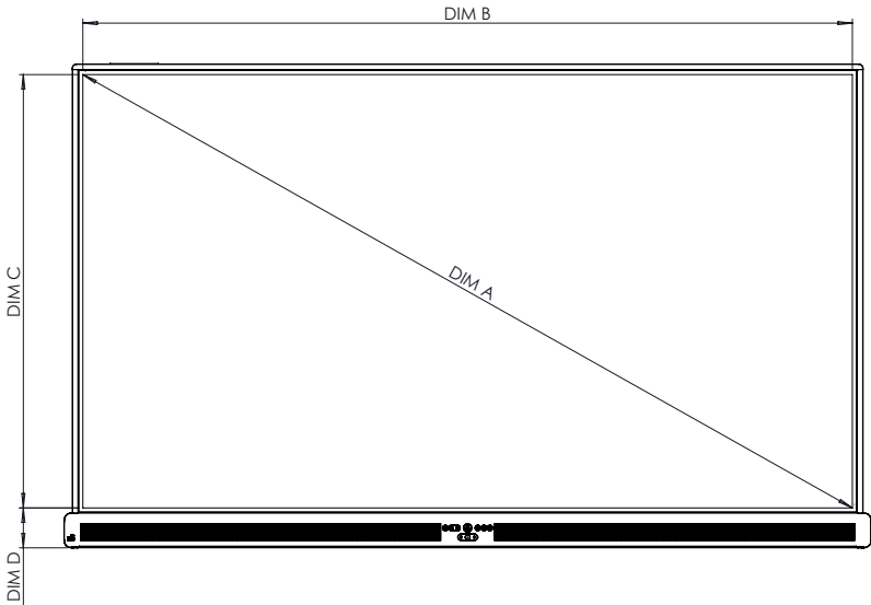
Vista frontal
